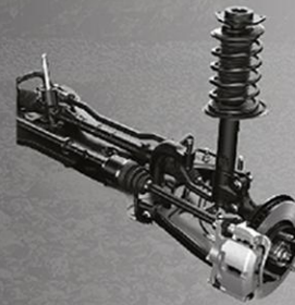
MacPherson Strut
